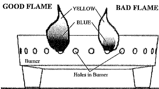
FLAME CHECK
